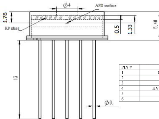
Pin description
