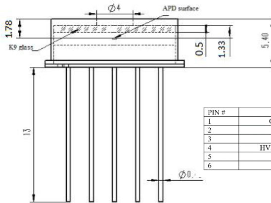
Pin description
