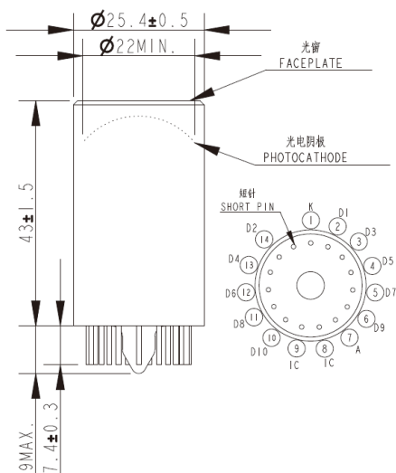
PMT structure
