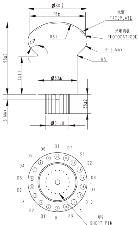
PMT structure
